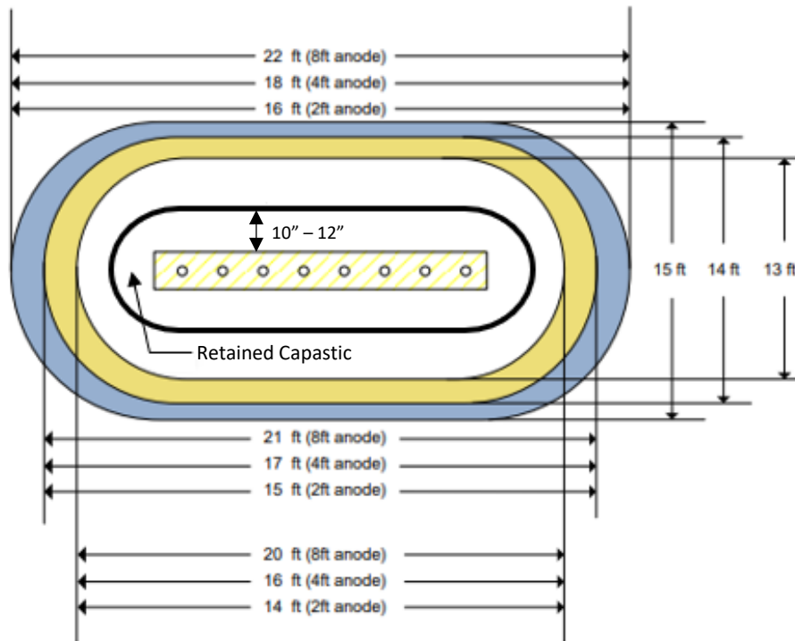
Figure E-1: Area to abrasive blast
