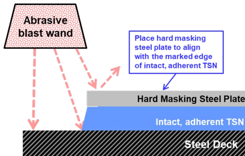
Figure B-4: Cross section view of masking alignment for abrasive blasting after HP WJ removal
