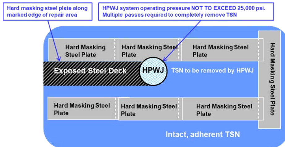
Figure B-2: Top view of hard masking plate configuration for HP WJ
