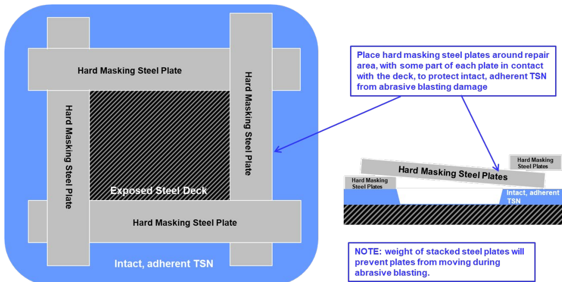
Figure B-3: Top view (left) and cross section view (right) of hard masking plate configuration around repair area
